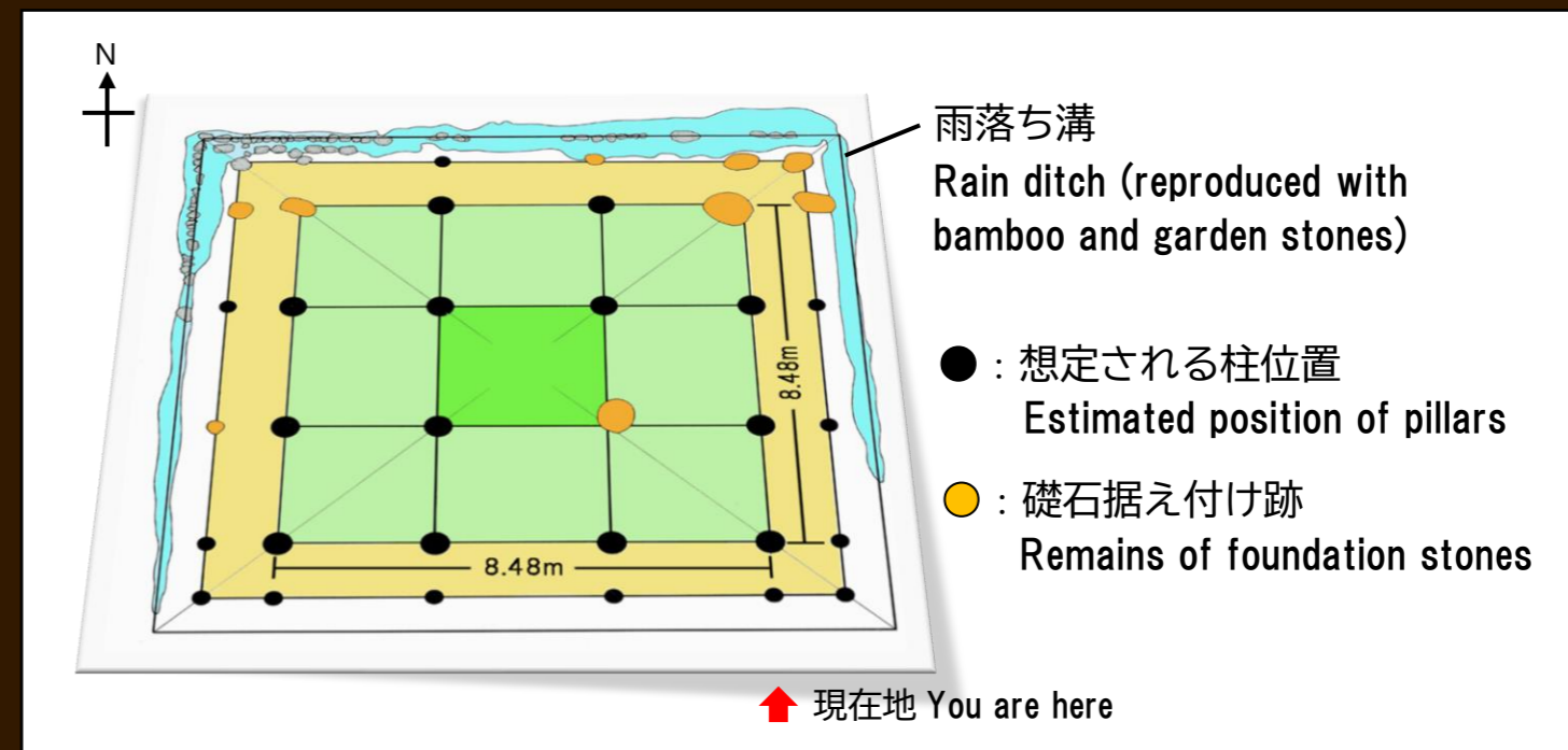
法華堂跡復元平面図 Ground plan of excavation results
